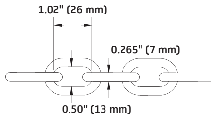
1/4" Grade 30 Chain
